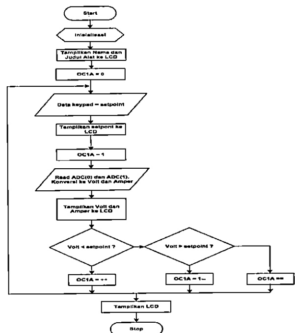
Gambar 32 : Flowchart Program Alat Boost Converter
