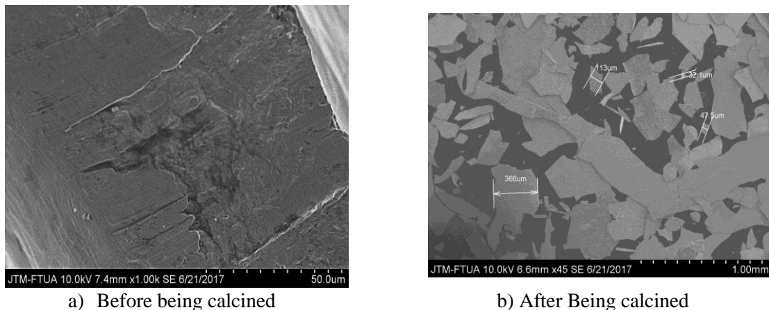
Figure 3. SEM Characterization [22-23]
