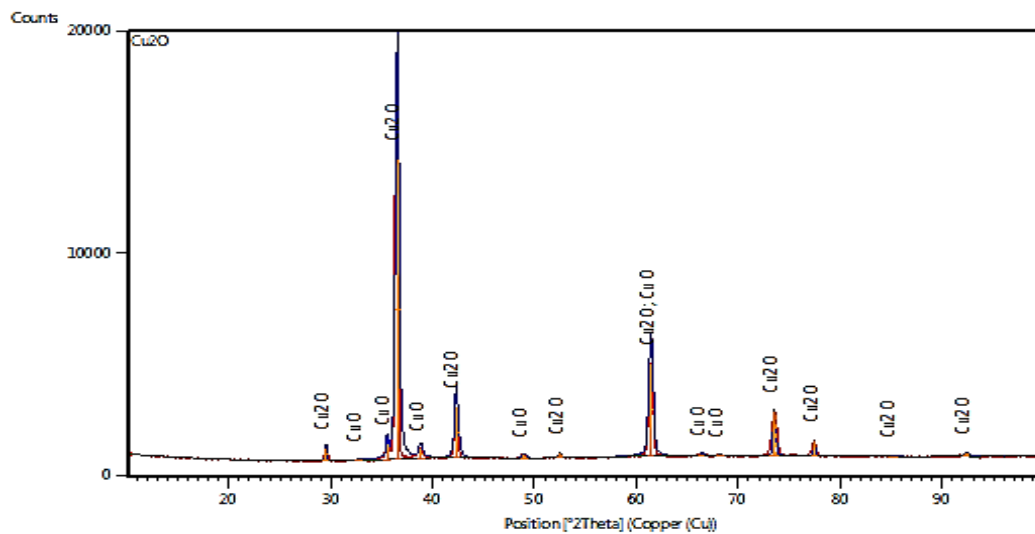
Figure 2. XRD Characteristics [29]
