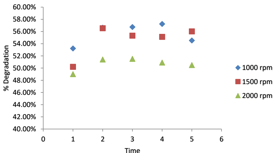
Figure 4. Effect of rotary speed and illumination time for degradation
