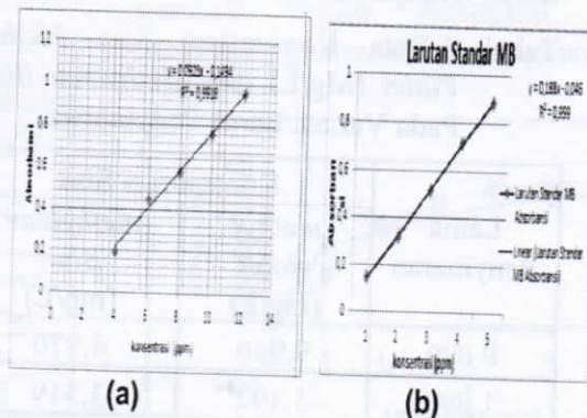
Gambar 1. Kurva Standar (a) Methyl Violet , Dan (B) Methylene Blue
