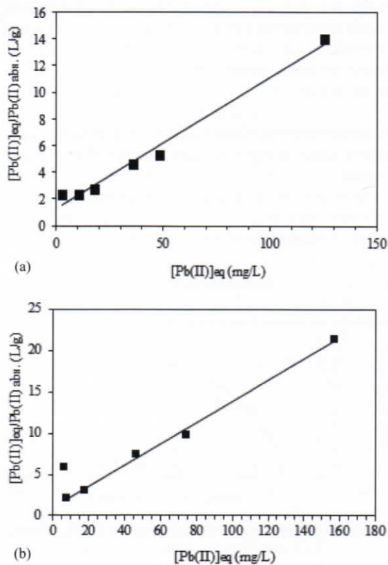
Gambar 6. Kurva Linieritas Langmuir biosorpsi logam timbal (II) (a)biomassa bsmosil dan (b) biomassa bsmonil
