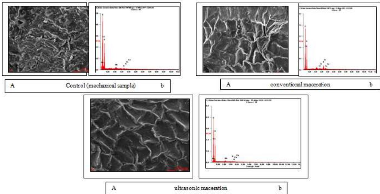
Fig. 4 Glucmannan granule size at 20 μm (a) Spectrum Shaping Elements granules (b). Porang flour optimization results purification
