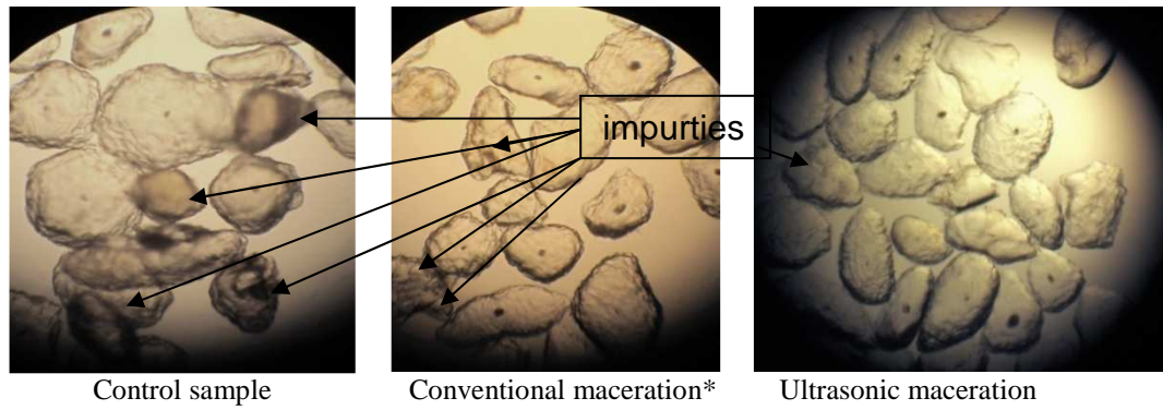
Fig.3 Light microscope magnification of 100 x observation of porang flour * [21]
