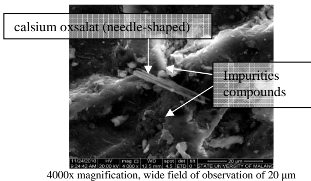
Fig. 5 SEM observation of needle-shaped oxalic acid crystals
