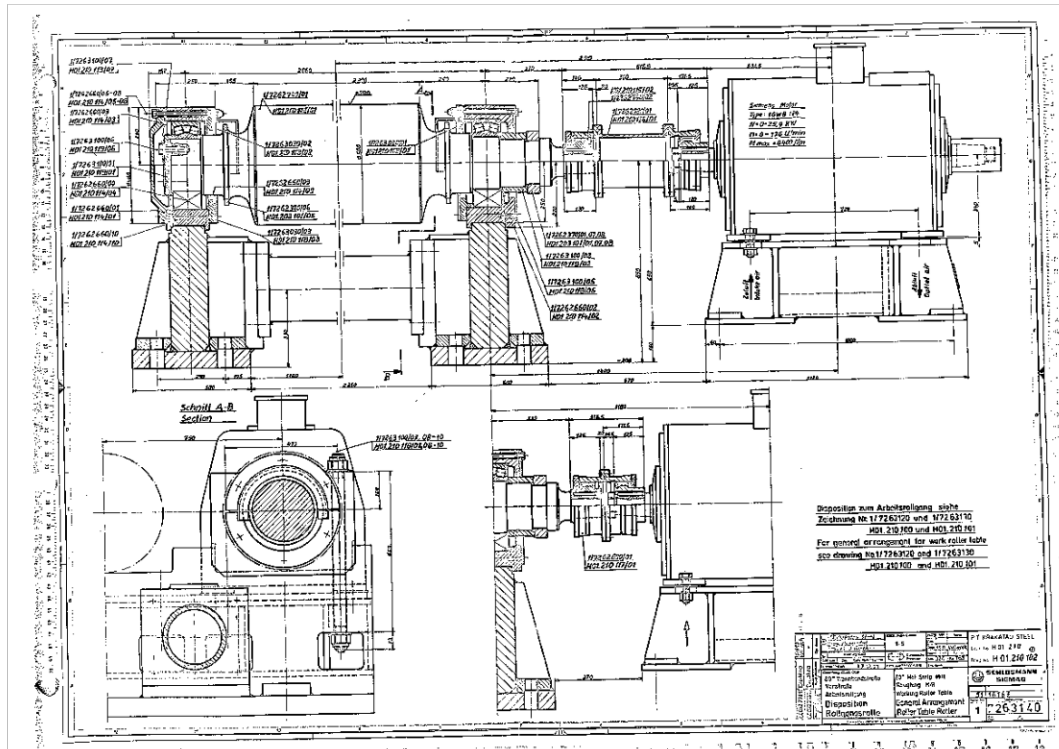
Gambar 5.1 Working Roller Table
