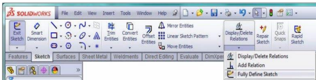
Gambar 4.16 Fitur Solidwork
