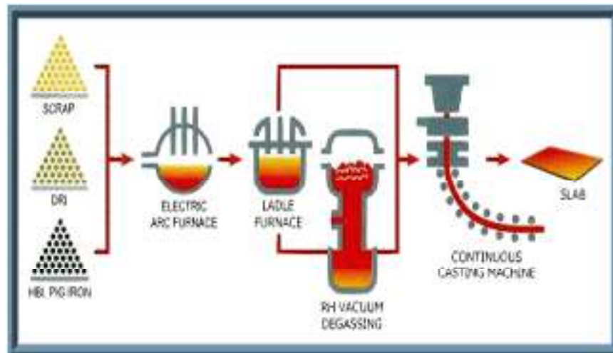
Gambar 2.8 Alur Proses produksi slab steel plant
