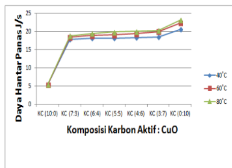
Figure 4 . Heat conductivity test graph
