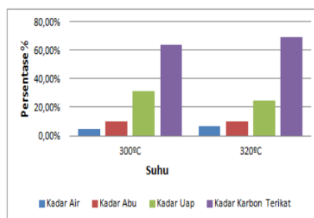
Figure1 .Graph of cassava peel carbonization temperature variations
