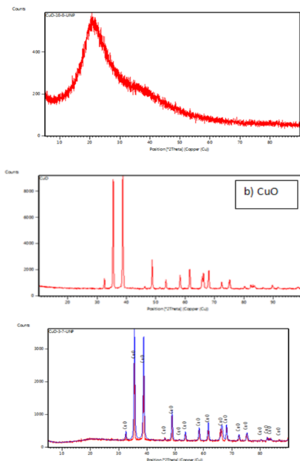
Figure 8 . (a) XRD spectrum of activated carbon, (b) Spectrum of CuO, (c) Conposit spectrum of activated carbon of CuO (3: 7)
