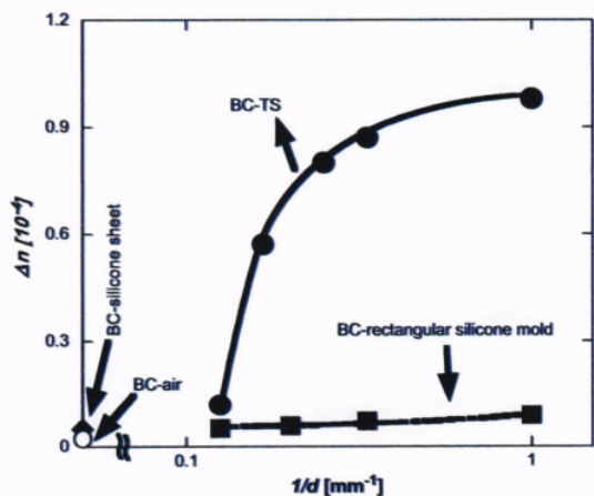
Fig. 7. The dependence of the birefringence ( \Delta n ) of BC–TS on the curvature of the silicone tube ( 1/d ) in which BC was cultivated (●). The wall thickness of the silicone tube was 1 mm. BC–SS (◆), BC produced on the 1-mm-thick silicone sheet; BC–air (○), BC produced at the liquid–air interface; and (■), BC produced in the 1-mm-thick rectangular silicone mold are also shown in the figure for comparison ( d , diameter of the silicone tube or the width of the rectangular mold).
