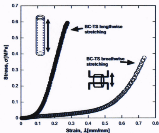
Fig. 6. Tensile stress–strain curves of the lengthwise (●) and breathwise (○) stretching of BC–TS produced in the silicone tube with an inner diameter and wall thickness of 6 mm and 1 mm, respectively. The duration of incubation was 3 days.
