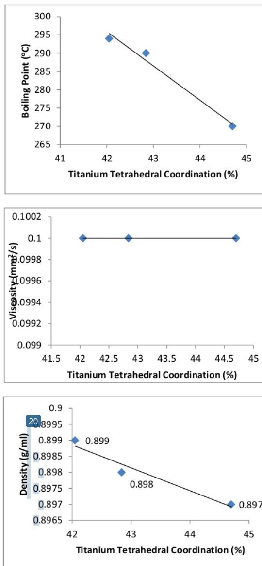
Fig.3. Effect of titanium tetrahedral fraction on physical properties of synthesized biodiesel with respect to boiling point, viscosity, and density.
