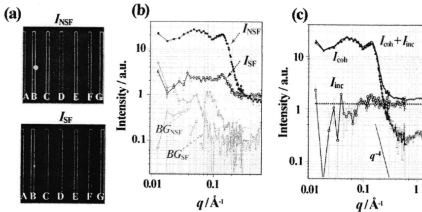
Fig. 2. (a) 2-dimensional distribution of the neutrons scattered from the water-swollen Nafion sample on the detector plane with the size of 250\text{mm} \times 250\text{mm} , with \Phi = 4^\circ . The color brightness corresponds to the frequency of neutron counting rate. The upper and lower images were obtained for the NSF and SF setups, respectively. The letters A to G indicate the position of the outlet of the corresponding benders, A to G. The white rectangular frames indicate the effective area, used for the analysis. (b) Totally averaged one-dimensional scattering profiles as a function of q . I_{NSF} (red filled circle) and I_{SF} (blue open circle) indicate the sample's profile measured at the NSF and SF setups, respectively. BG_{NSF} (light red filled rectangle) and BG_{SF} (light blue open rectangle) are for the empty cell. (c) Separated coherent ( I_{coh} , red filled circles) and incoherent ( I_{inc} , blue open circles) scattering contributions, and the sum of the two ( I_{coh} + I_{inc} , purple line). The gray curve added in the high q side ( q > 0.5 \text{\AA}^{-1} ) indicates the profile obtained by use of unpolarized neutron beam. By subtracting the determined incoherent scattering (dashed gray line) from this, the coherent contribution (gray circles) was determined.
