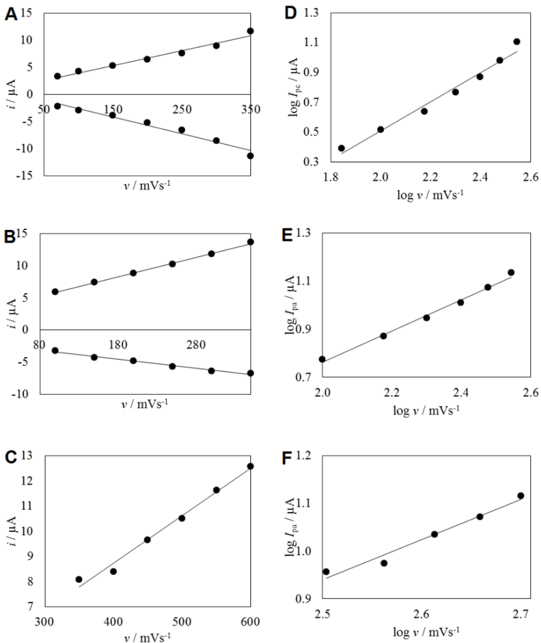
Figure 11. The graph of peak current versus scan rate for (A) DA, (B) ACT, and (C) BPA, and the graph of log peak current versus log scan rate for (D) DA, (E) ACT, and (F) BPA.
