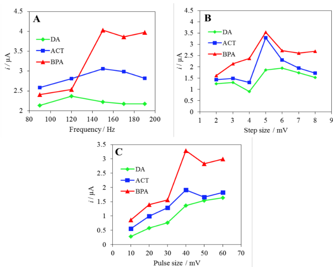
Figure 7. Effects of the SWV parameters (A) frequency, (B) step size, and (C) pulse size on current response. Solution: 1 \times 10^{-4} M DA, ACT and BPA mixture.
