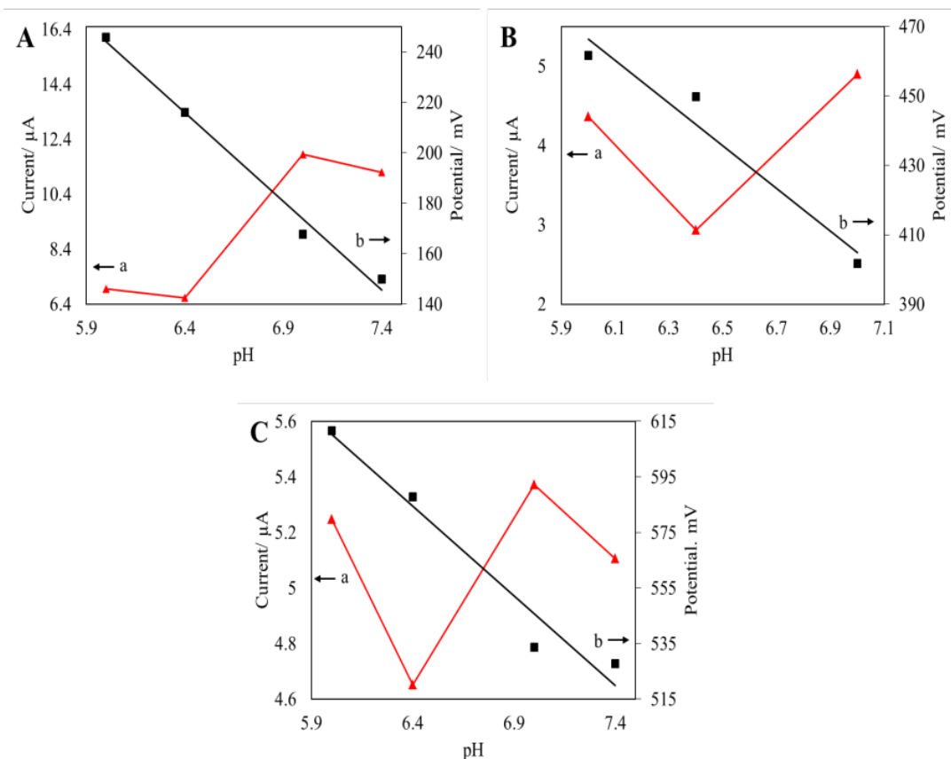
Figure 8. Graphs of current response (line a) and peak potential (line b) on varying pH value of (A) DA, (B) ACT, and (C) BPA solution.
