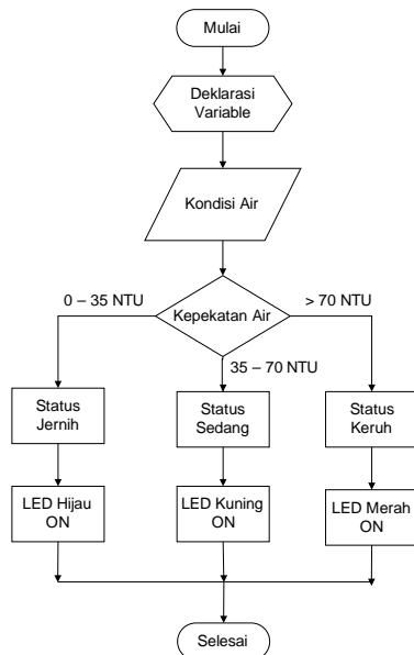
Gambar 6 Flowchart Rangkaian
