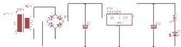
Gambar 5 Rangkaian Power Supply Regulator
