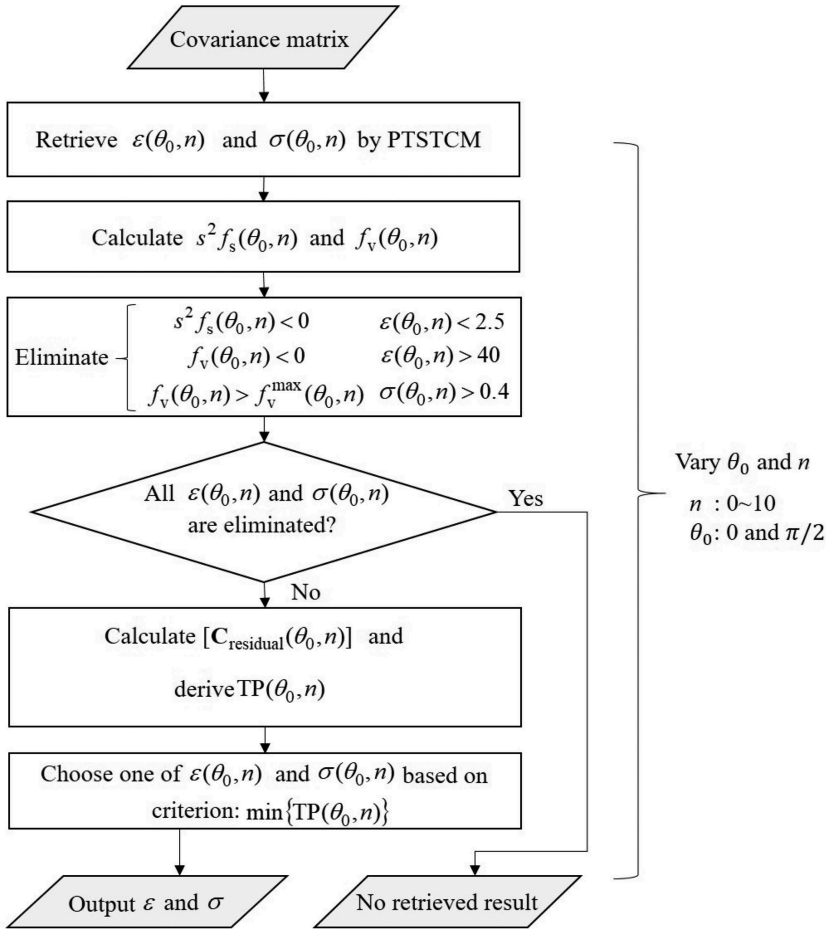
Figure 4. The adaptive PTSTCM algorithm.
