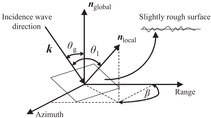
Figure 3. A geometry of a rotated single facet along both azimuth and range direction in the PTSM.
