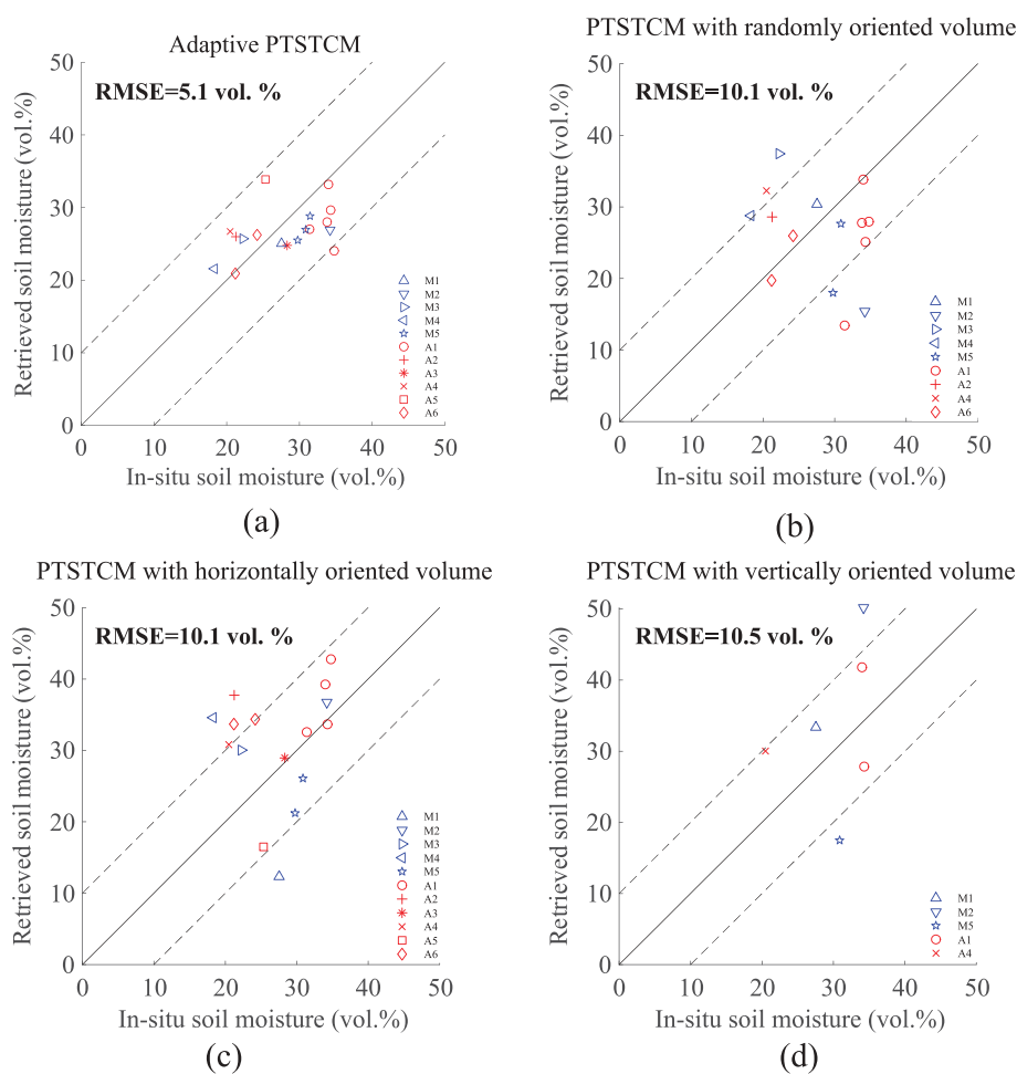
Figure 6. Scatter plots of retrieved soil moisture results versus in situ soil moisture results at 0–11 cm depth. The blue symbols show data on 25 March, whereas the red symbols show data on 2 August. (a) The adaptive PTSTCM; (b) The PTSTCM with randomly oriented volume; (c) The PTSTCM with horizontally oriented volume; (d) The PTSTCM with vertically oriented volume.
