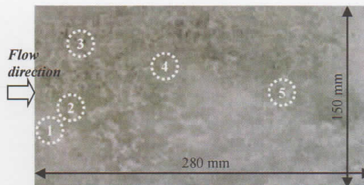
Fig. 3 Surface of concrete specimen (test type A) before pouring bio-based repair materials. Section marked with points where FT-IR observation will be spotted
